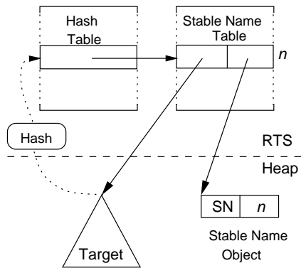
Fig. 2. Stable Name Implementation
